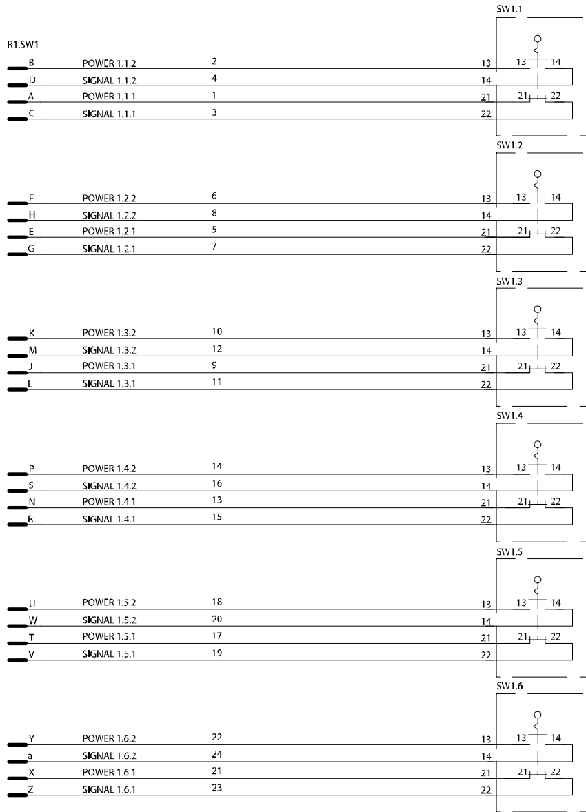
Switches axis 1
