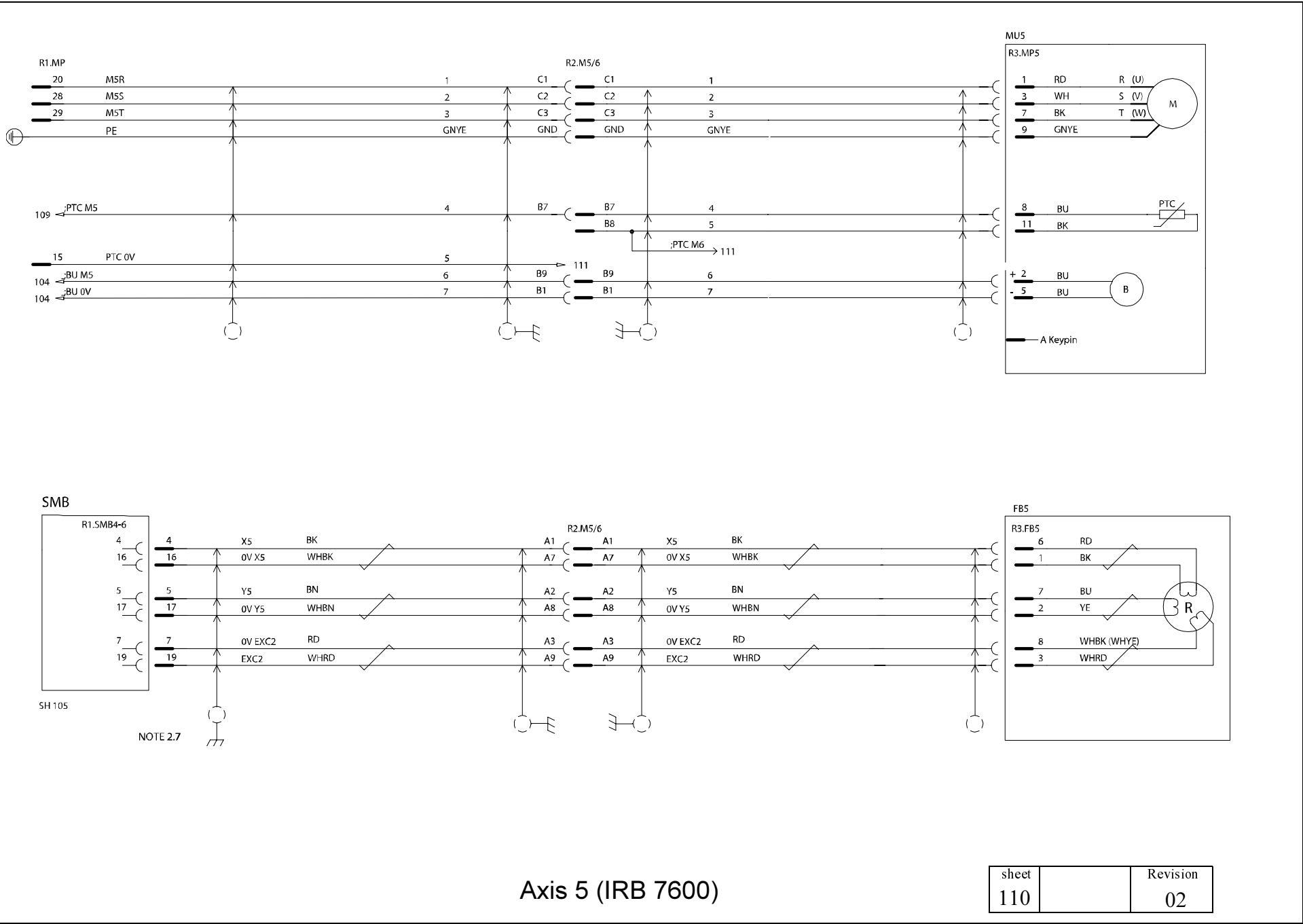
Circuit Diagram 3HAC 13347-1
